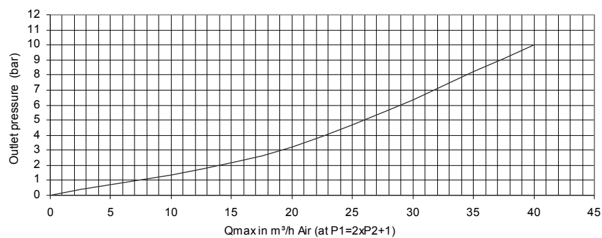
Flow performance E 86 - VA
